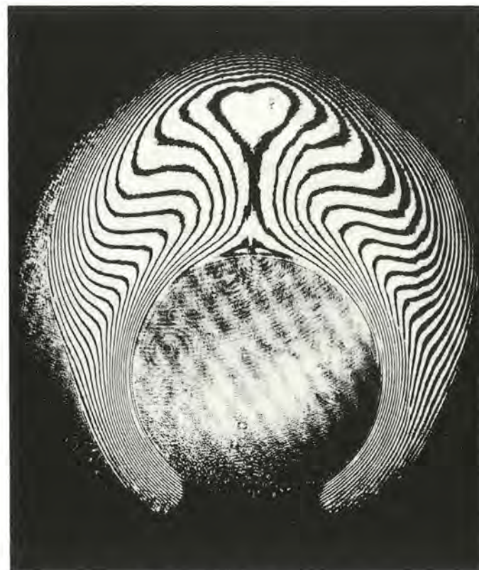
Heat transfer patterns on a circular tube
