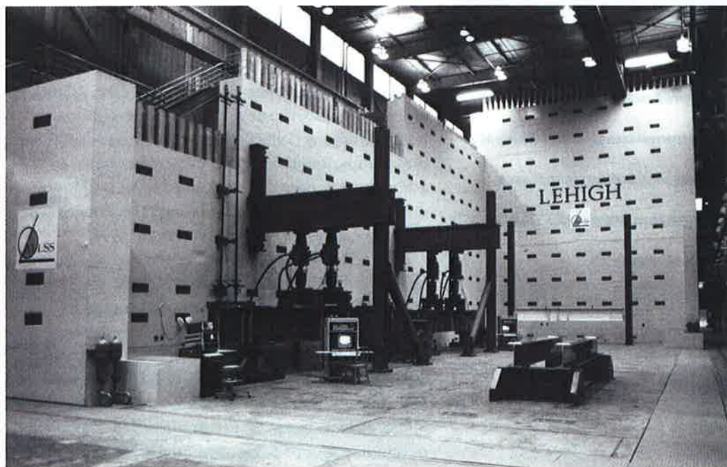
Lehigh ERC. The Multidirectional Experimental Laboratory, shown here, is at Lehigh University's Center for Advanced Technology for Large Structural Systems. Here full-scale structures are tested under multidirectional loads. The center is also investigating innovations in design concepts, fabrications and assembly techniques, and performance monitoring.
